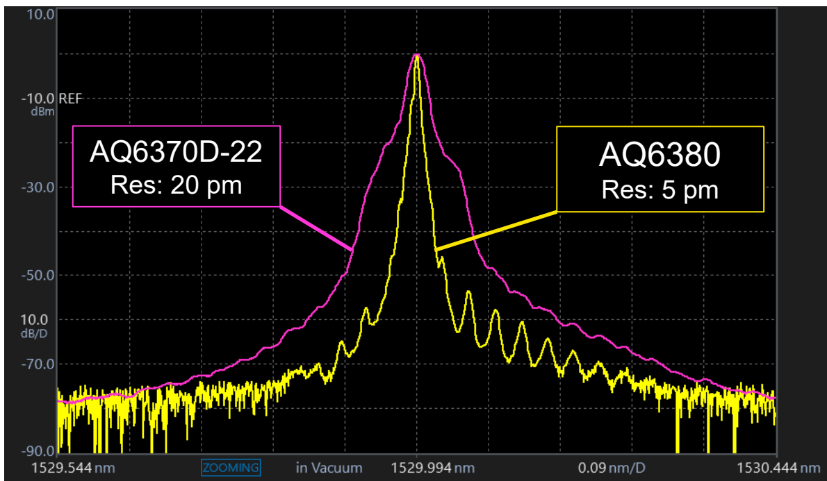
Spectrum of External Cavity Laser
